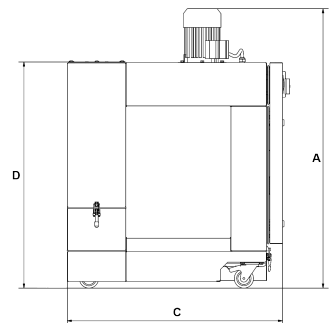
LEFT VIEW
