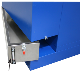
STAINLESS STEEL CONTAINER WITH WATER FOR SPARKS EXTINGUISHER
