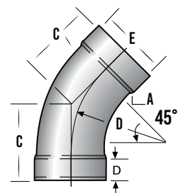
45° SHORT RADIUS ELBOW
